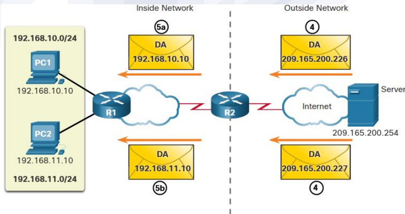
IPv4 NAT Pool
